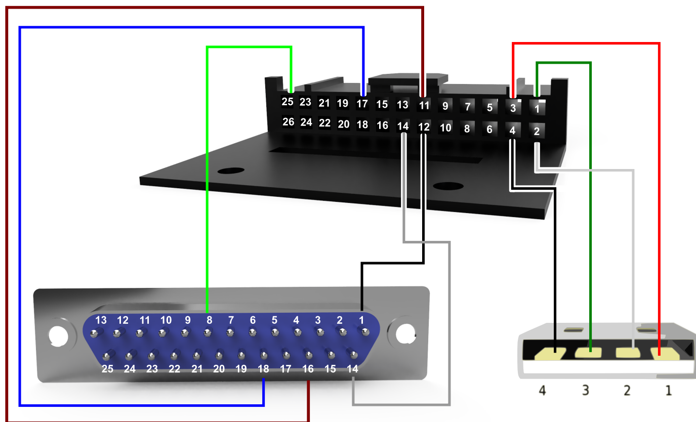
USB Type A
